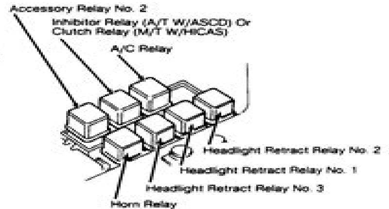
RELAY BOX
