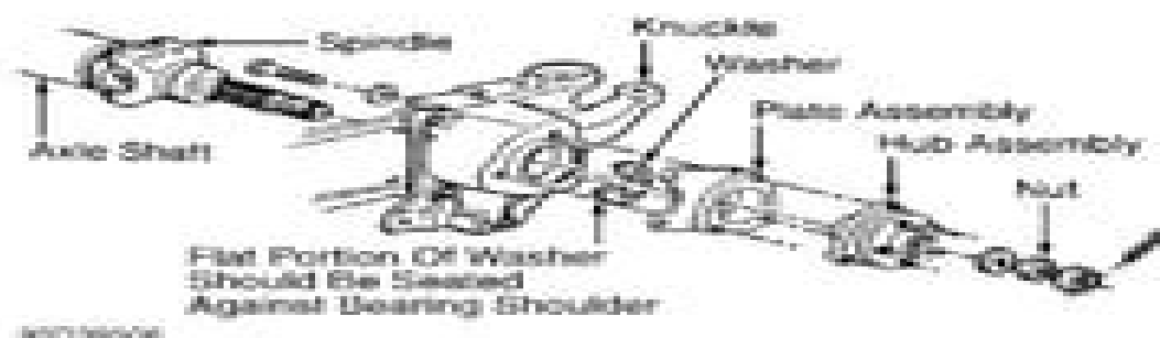
Fig. 1: Exploded View Of Knuckle & Hub Courtesy of GENERAL MOTORS CORP.
