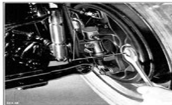
Fig. 68—Turning Brake Shoe Cam
