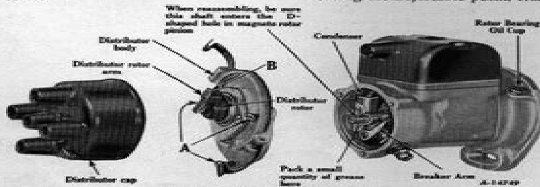
Illustr. 54—Magneto Disassembled
