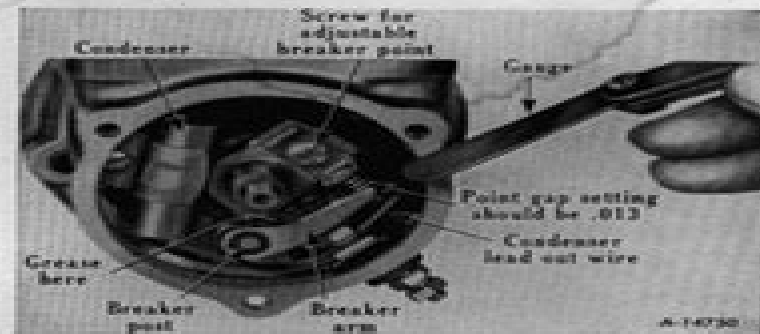
Illustr. 53—Adjusting the Breaker Points.
