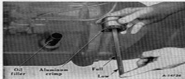
Illustr. 18—Checking the Oil Level in the Crankcase.
