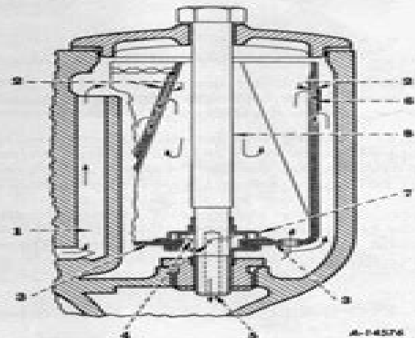
Illustr. 19—Cutaway view of filter showing: (1) oil inlet, (2) replaceable filtering element, (3) mesh screen separator to provide passage for filtered oil between inner and outer layer of element, (4) outlet for filtered oil, (5) filtered oil return, (6) band holding folds of element together, (7) oil seal, (8) stud.
