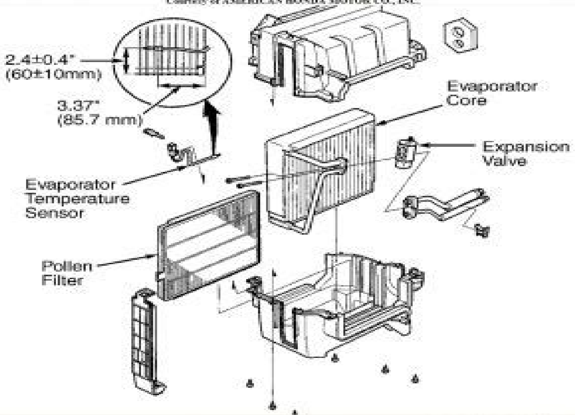
Fig. 21: Identifying Evaporator Components Courtesy of AMERICAN HONDA MOTOR CO., INC.
