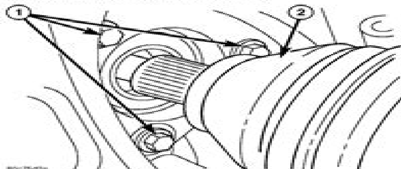
Fig. 14 HALFSHAFT / HUB/BEARING
