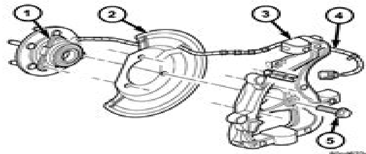
Fig. 15 HUB/BEARING 4X2
