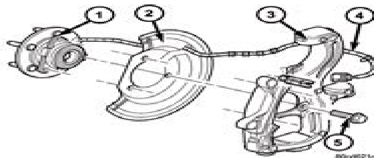
Fig. 16 HUB/BEARING 4X4
