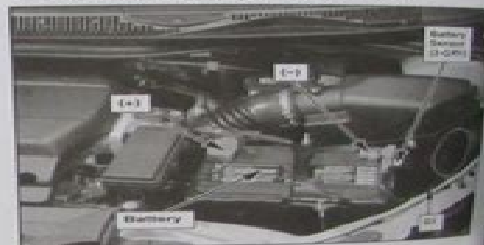
17. Left Side of Engine Compartment
