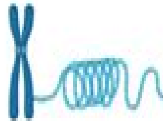
Chromosome and condensed chromatin
