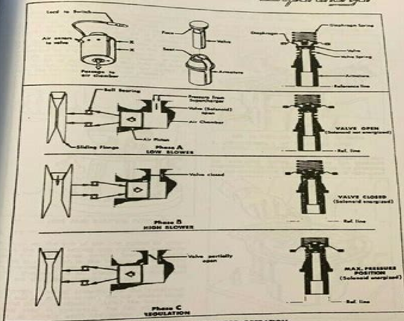
FIG. 12 SOLENOID REGULATOR OPERATION
