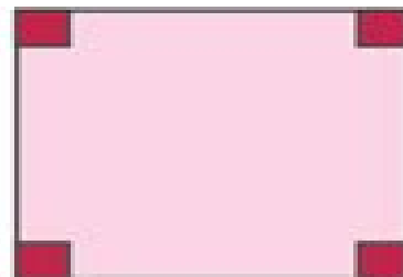
Square
