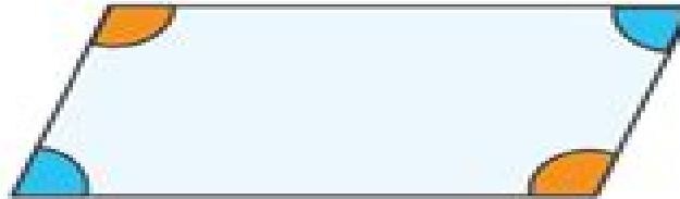
Parallelogram
