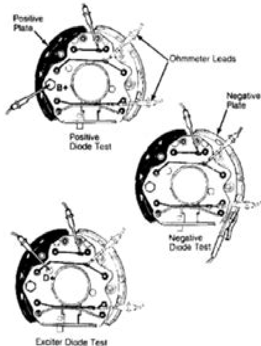
Fig. 1: Bosch Diode Assembly Test
