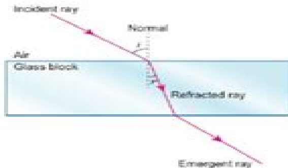
Figure 6.2 Refraction of light
