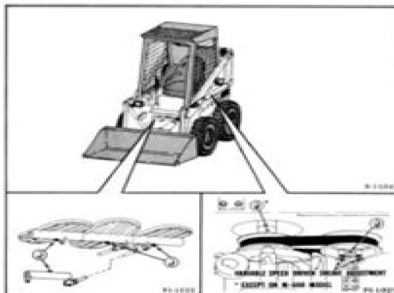
Fig. 5-2 Loader Lubrication
