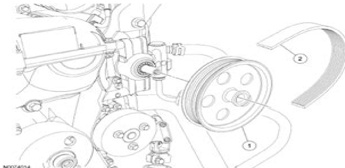
Fig. 10: Identifying Power Steering Pump Pulley - 2.3L. Courtesy of FORD MOTOR CO.
