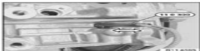
Fig. 157: Securing Crankshaft Using Special Tool (11 0 300)
