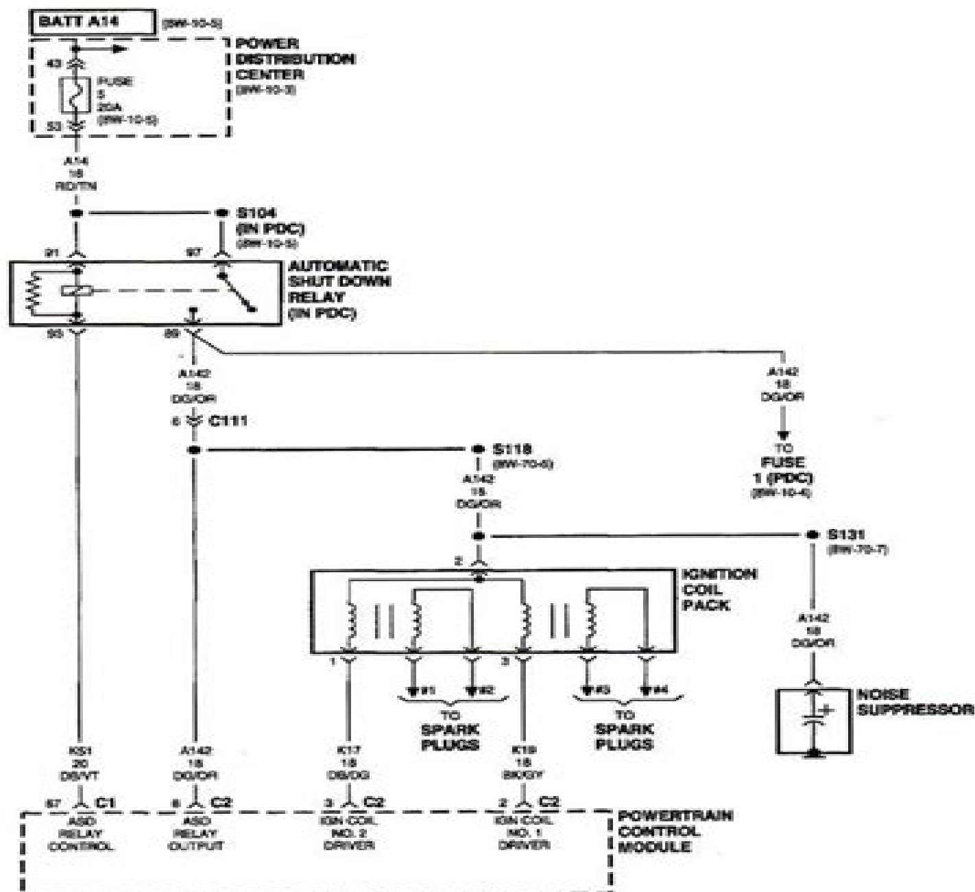
Fuel/Ignition System
