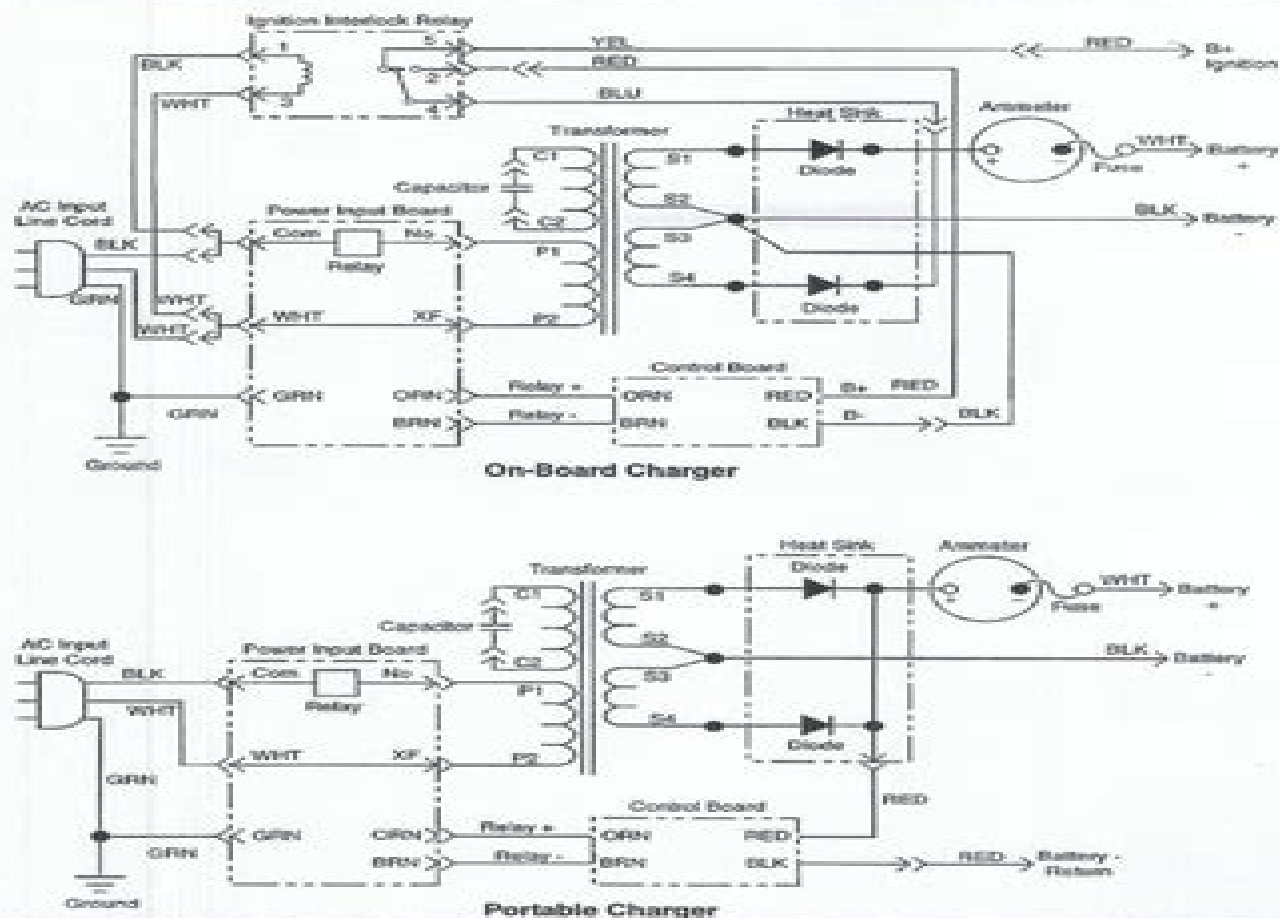
Fig. 5 PowerWise™ Charger Wiring Diagrams
