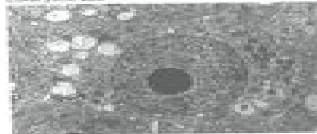
Eukaryotic cell
