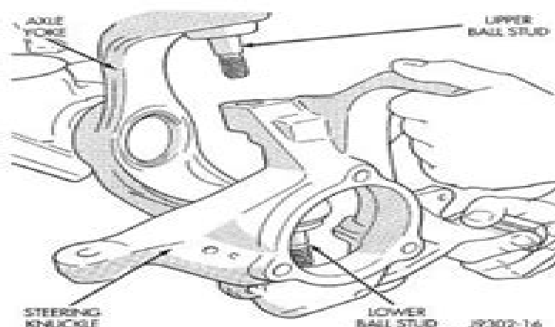
Fig. 22 Steering Knuckle Removal/Installation
