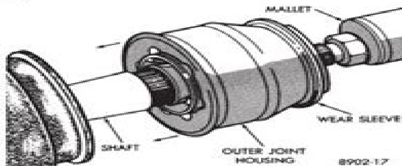
Fig. 21 Joint Installation
