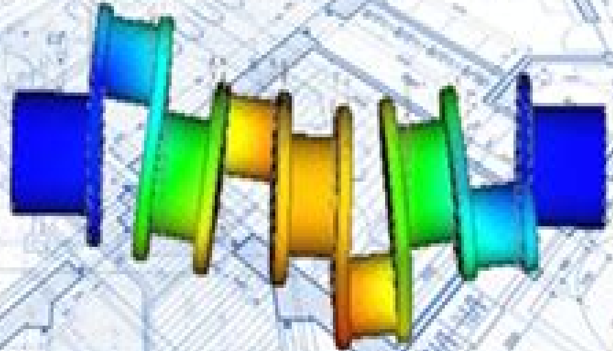
Mode Shape 1 - Frequency 104.6 Hz
