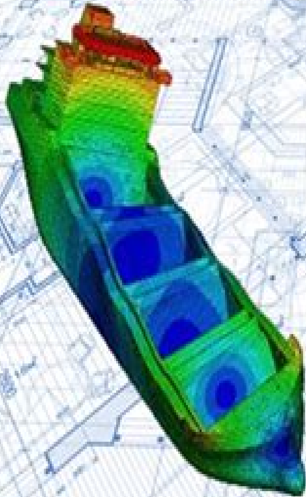
Mode Shape 2 - Frequency 151.7 Hz
