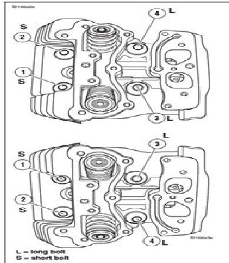
Figure 3-38. Cylinder Head Bolt Torque Sequence
