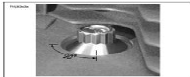
Figure 3-39. Final Tightening For Cylinder Head Bolts
