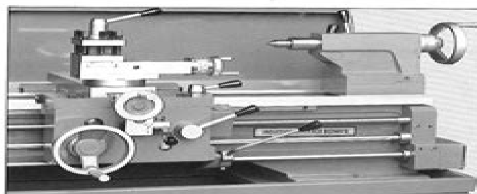
APRON & CARRIAGE
