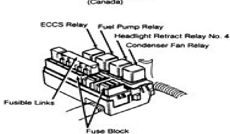
FUSE/RELAY BLOCK
