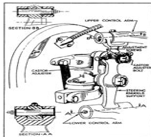
Fig. 53. Knuckle Support
