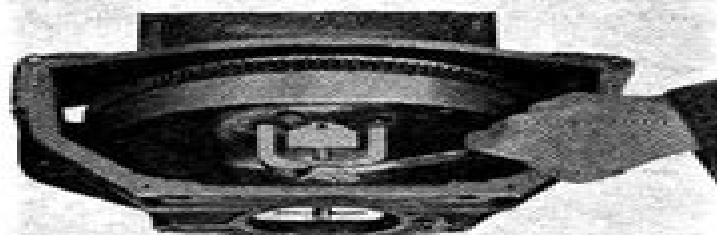
Fig. 84—Clutch Pilot Bearing Puller—Master Models
