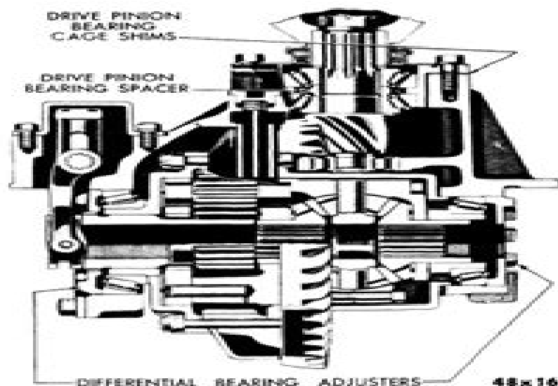
Fig. 46—Rear Axle Differential Two-Speed Spiral Bevel (Assembled View)
