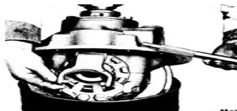
Fig. 48—Removing or Installing Shift Fork and Shaft
