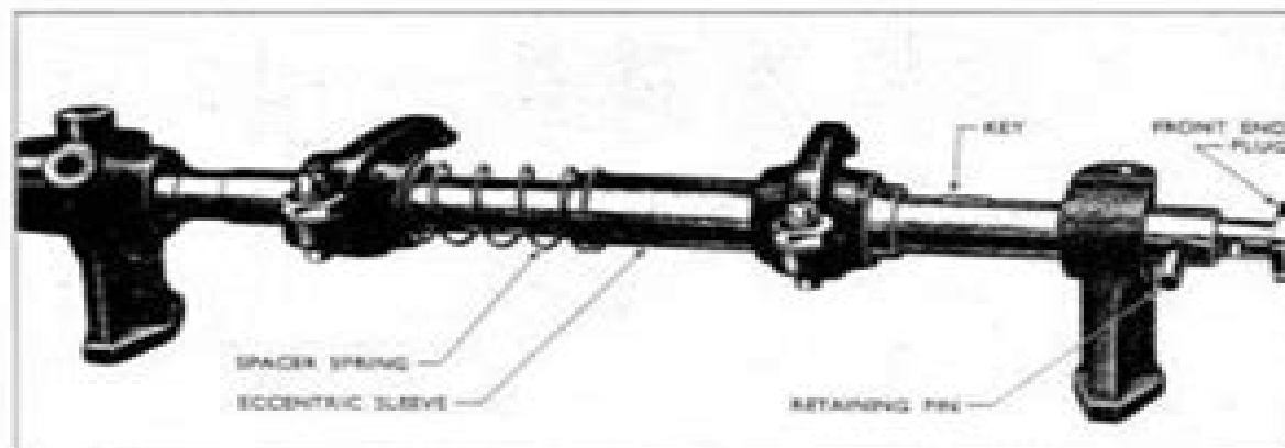
Fig. 1 Rocker Shaft and Supports
