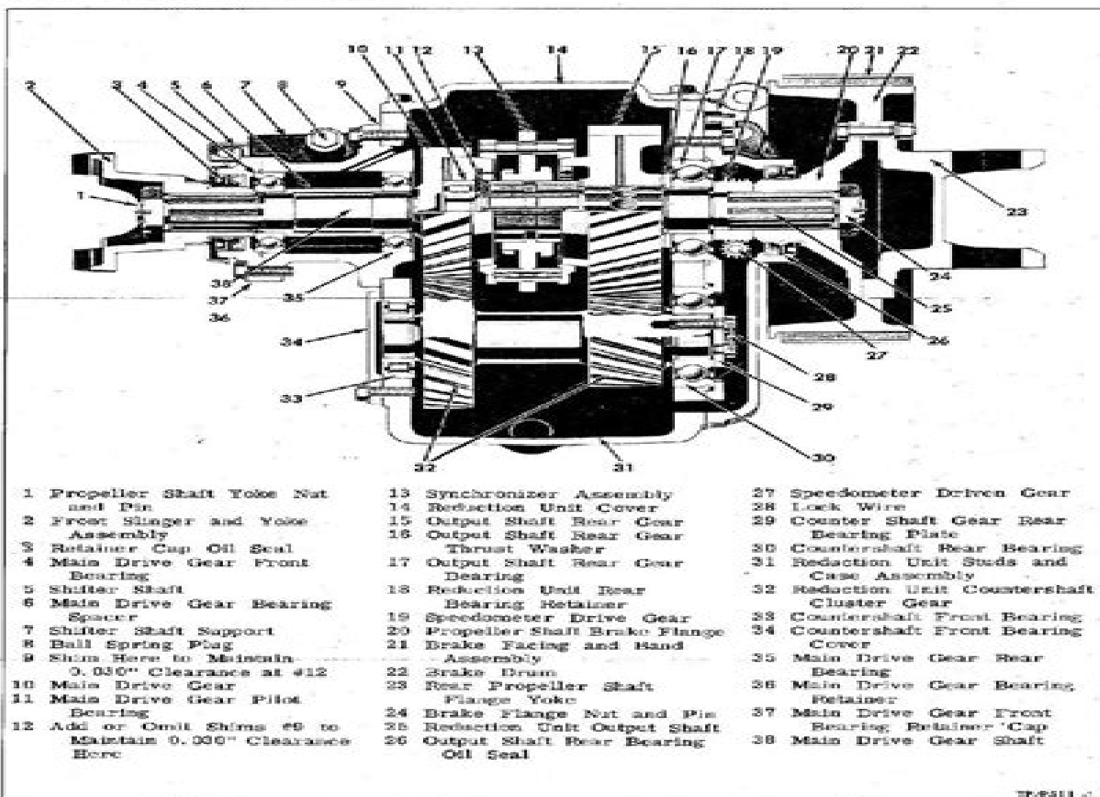
Figure 162—Two-Speed Reduction Unit (Series M350-24 Through M470-30 Only)
