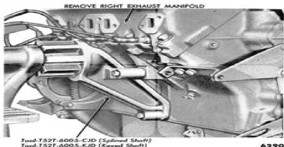
Fig. 5—Engine Mount—302 or 332 Cubic Inch Engine
