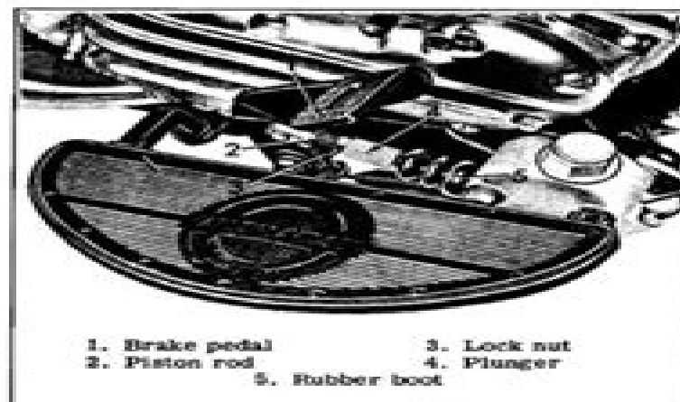
Figure 2G-7. Adjusting Rear Brake Pedal
