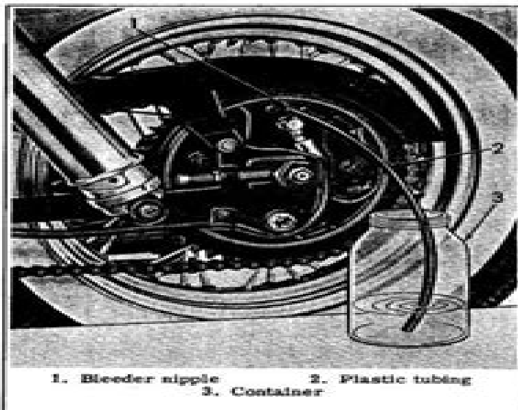
Figure 2G-6. Bleeding Hydraulic Brake System
