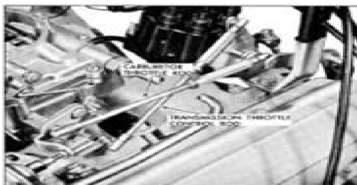
Fig. 6B-3 Carburetor Throttle Linkage (H/M shown)
