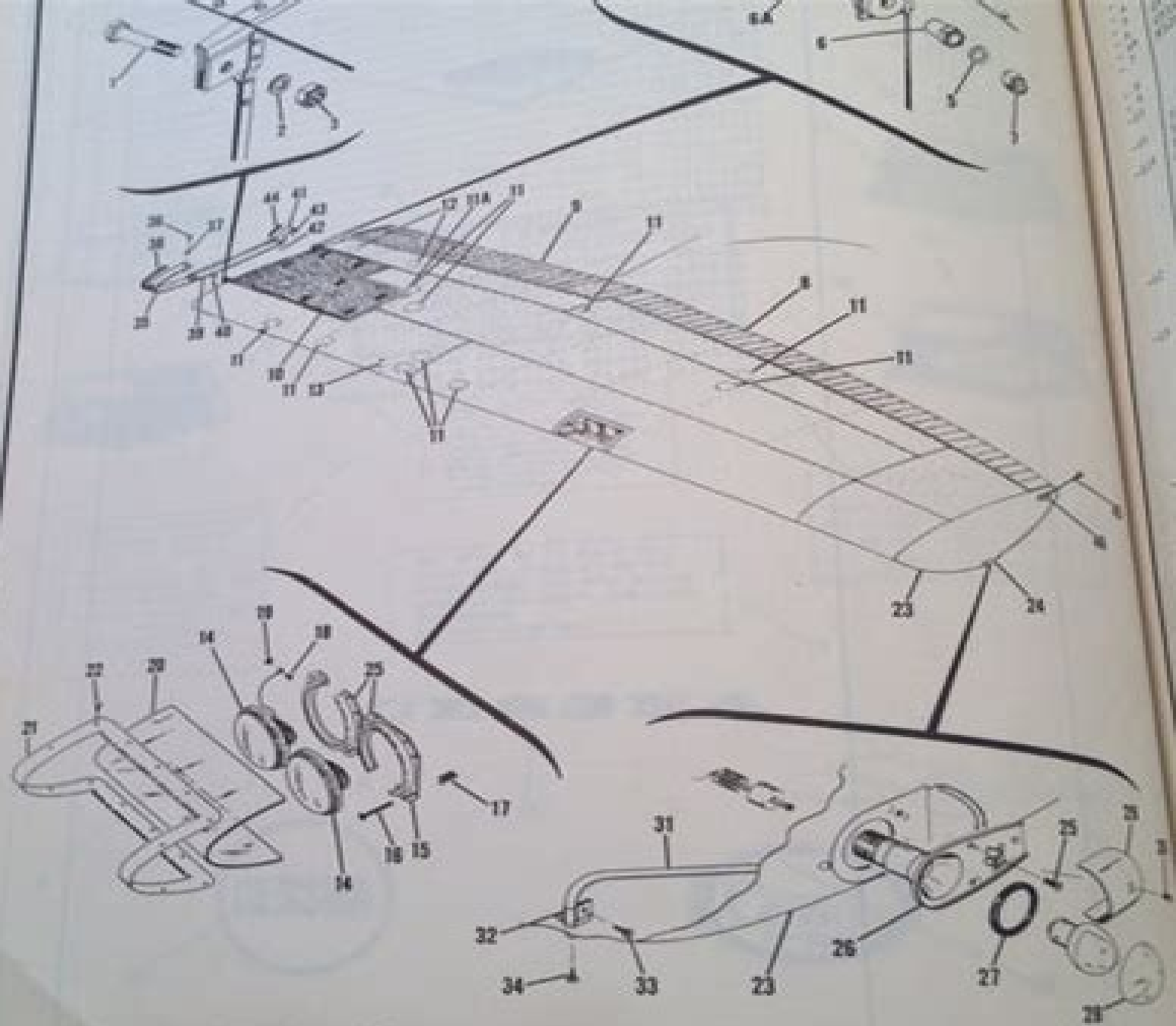
Figure 3. Wing Assembly Complete
