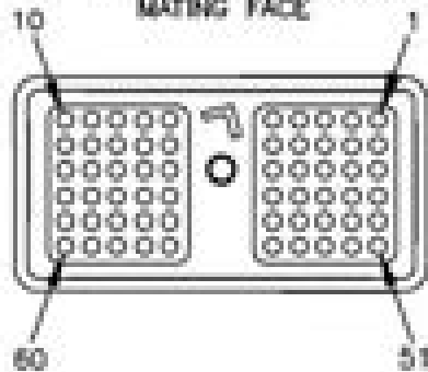
ENGINE HARNESS CONNECTOR MATING FACE
