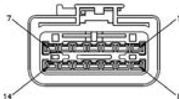
AFTERTREATMENT INTERFACE CONNECTOR MATING FACE
