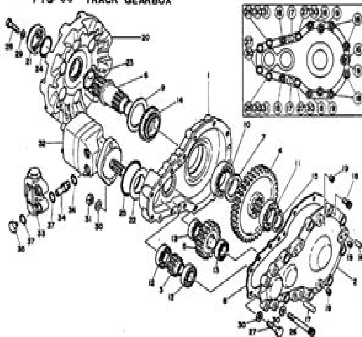
FIG 06 TRACK GEARBOX
