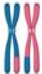
Chromosomes (recombinant)
