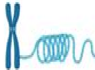
Chromosome and condensed chromatin
