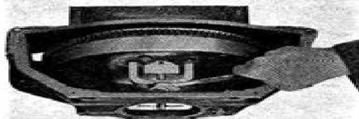
Fig. 84—Clutch Pilot Bearing Puller— Master Models
