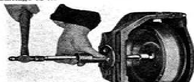
Fig. 85—Clutch Pilot Bearing Installer— Master Models
