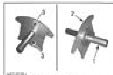
FIGURE 1 1. Alignment shaft support PN 525 035 500 2. Alignment shaft PN 288 000 145 3. M6 x 25 x 1,25 hexagonal screws
