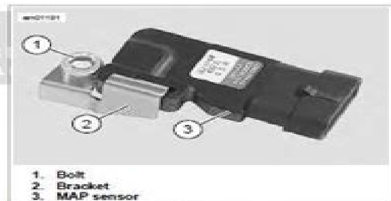
Figure 4-14. MAP Sensor
