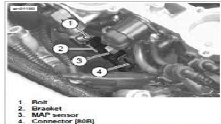
Figure 4-13. MAP Sensor Location (typical)
