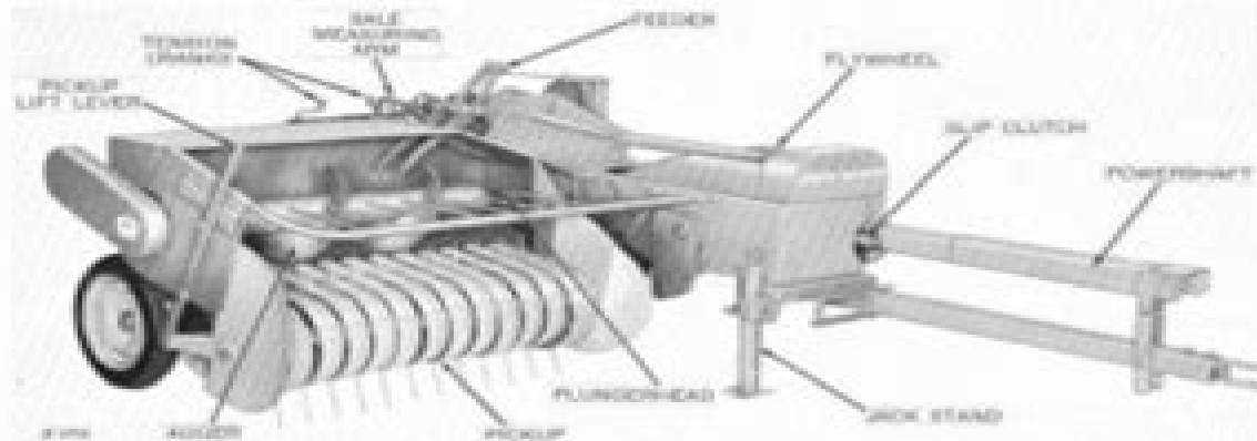
John Deere D4T Baler with Power Take-Off
